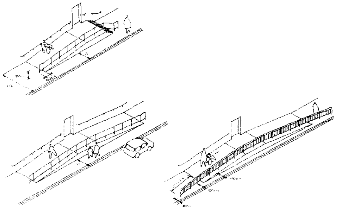
Figure 20 Ramp Dimension
