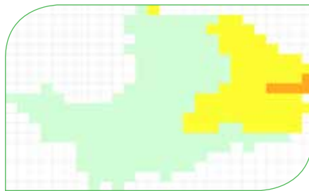
2008 Annual Mean PM 10 Concentration (2006 Base Year)
