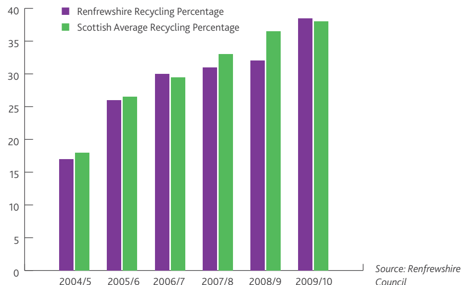
Fig 5.6 - The % level of recycling within Renfrewshire since 2004
