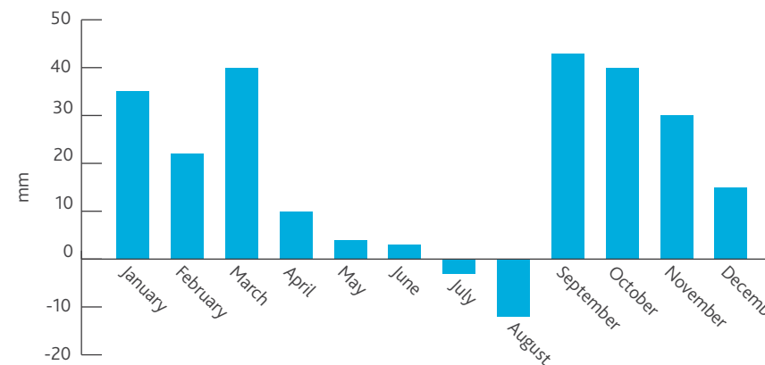
Fig 8.3: Paisley: Change in Mean Monthly Rainfall (1890–2009)
